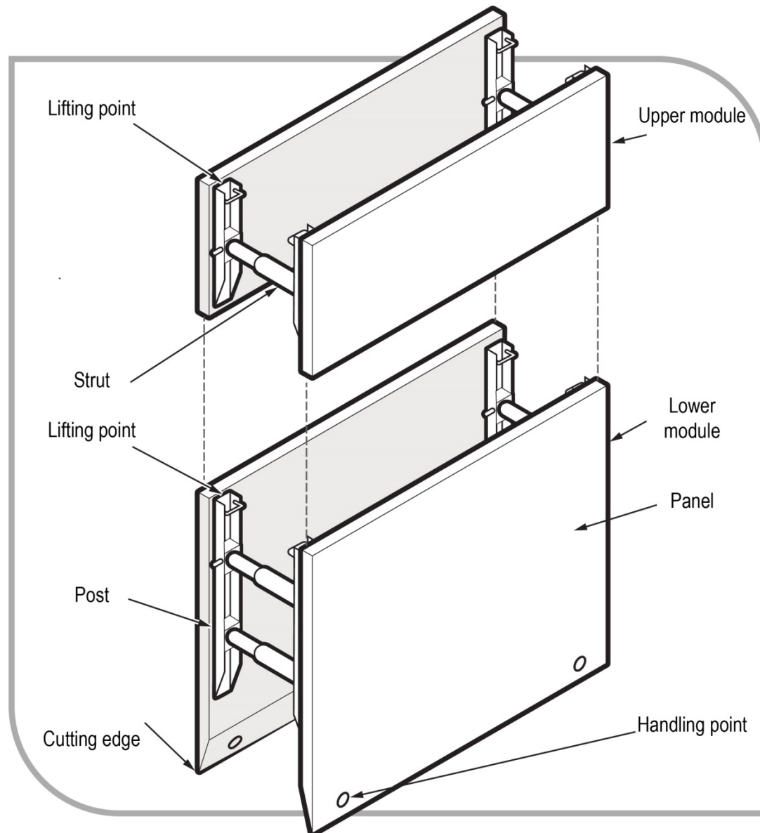
Figure 19 Typical trench shield
