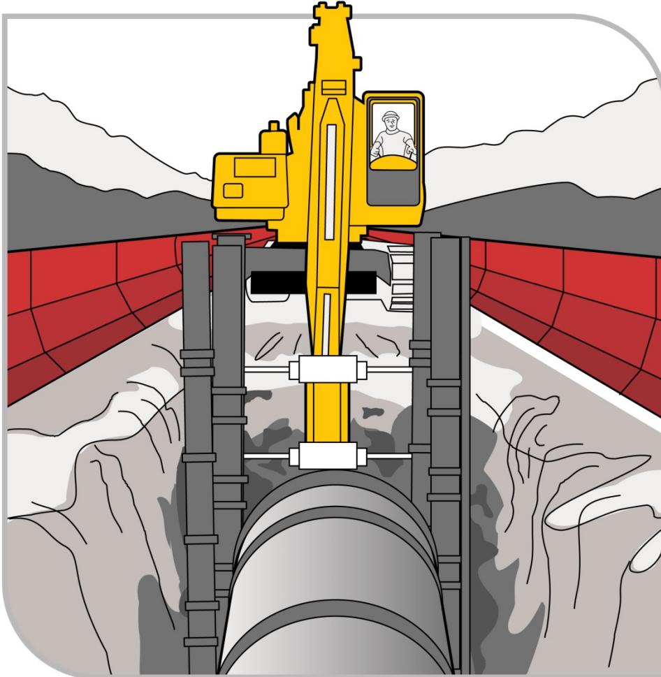
Figure 6 Extending trench shields above the excavation
