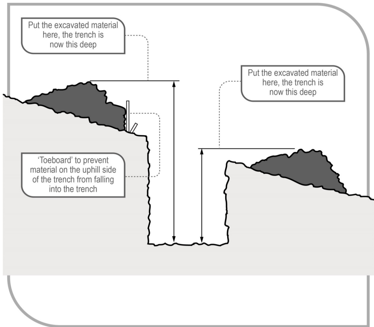
Figure 3 Excavated material impact on effective excavation depth
