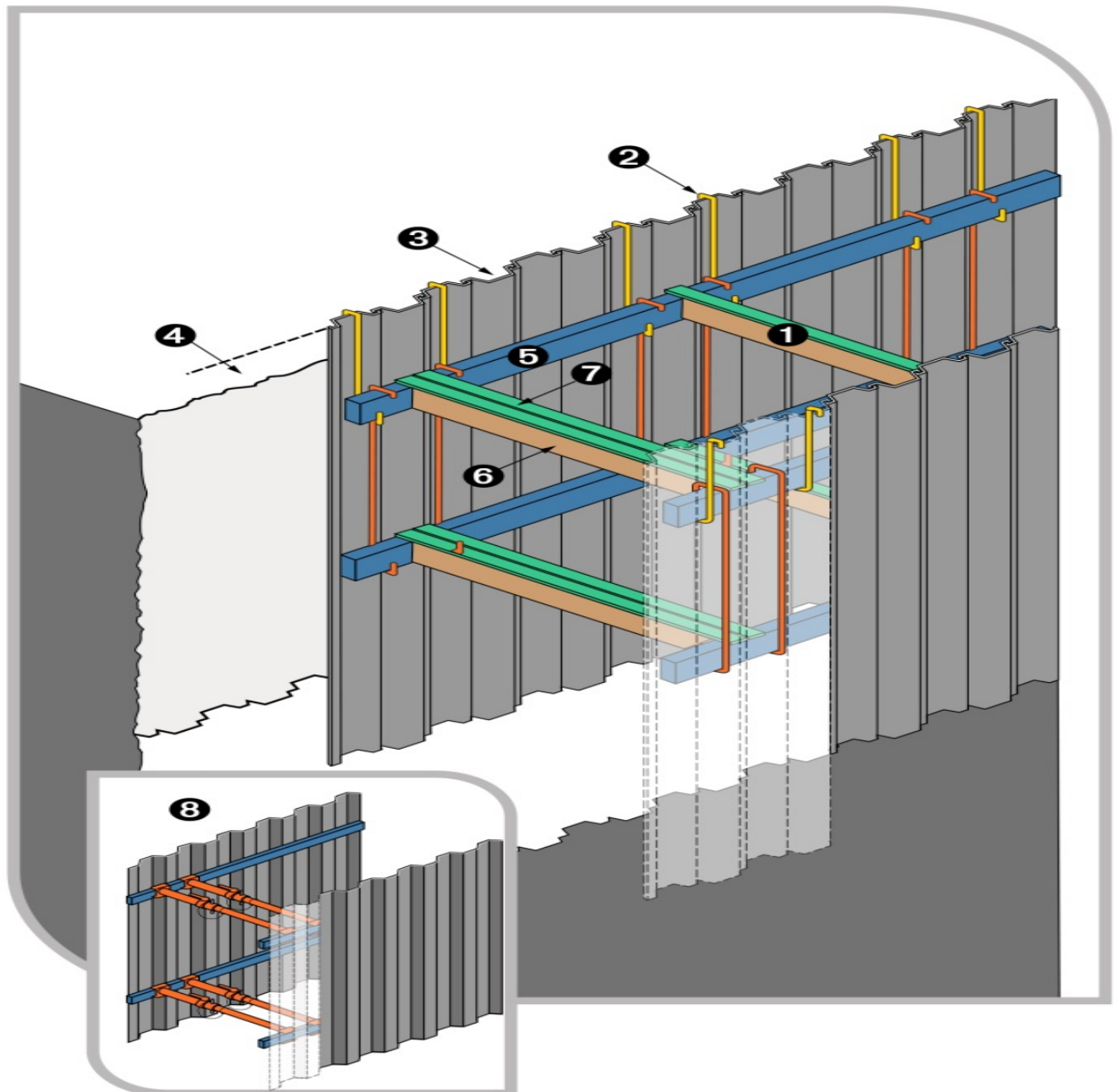
Figure 13 Steel sheet piling
