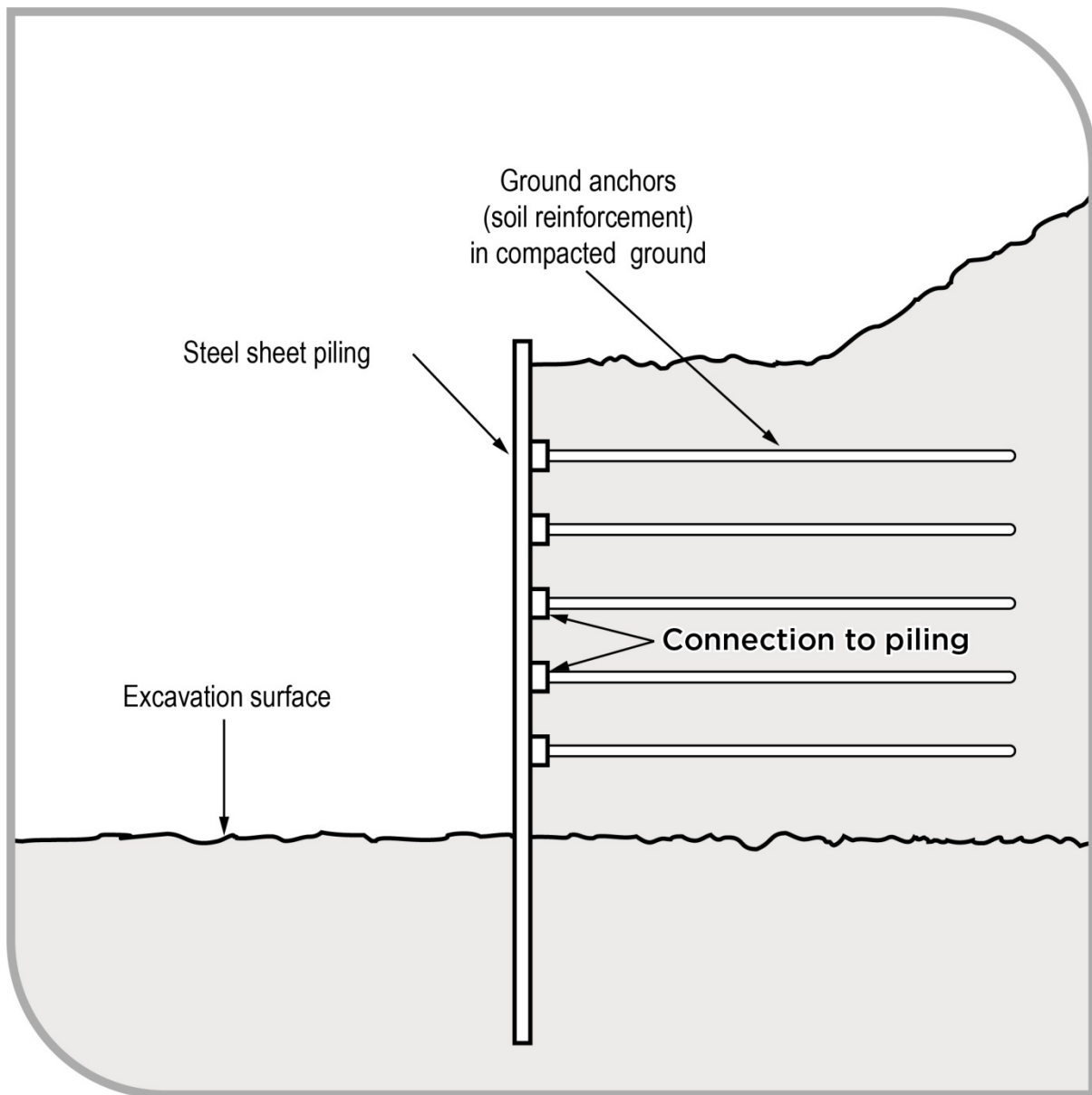
Figure 18 Ground anchors for supporting steel sheet piling
