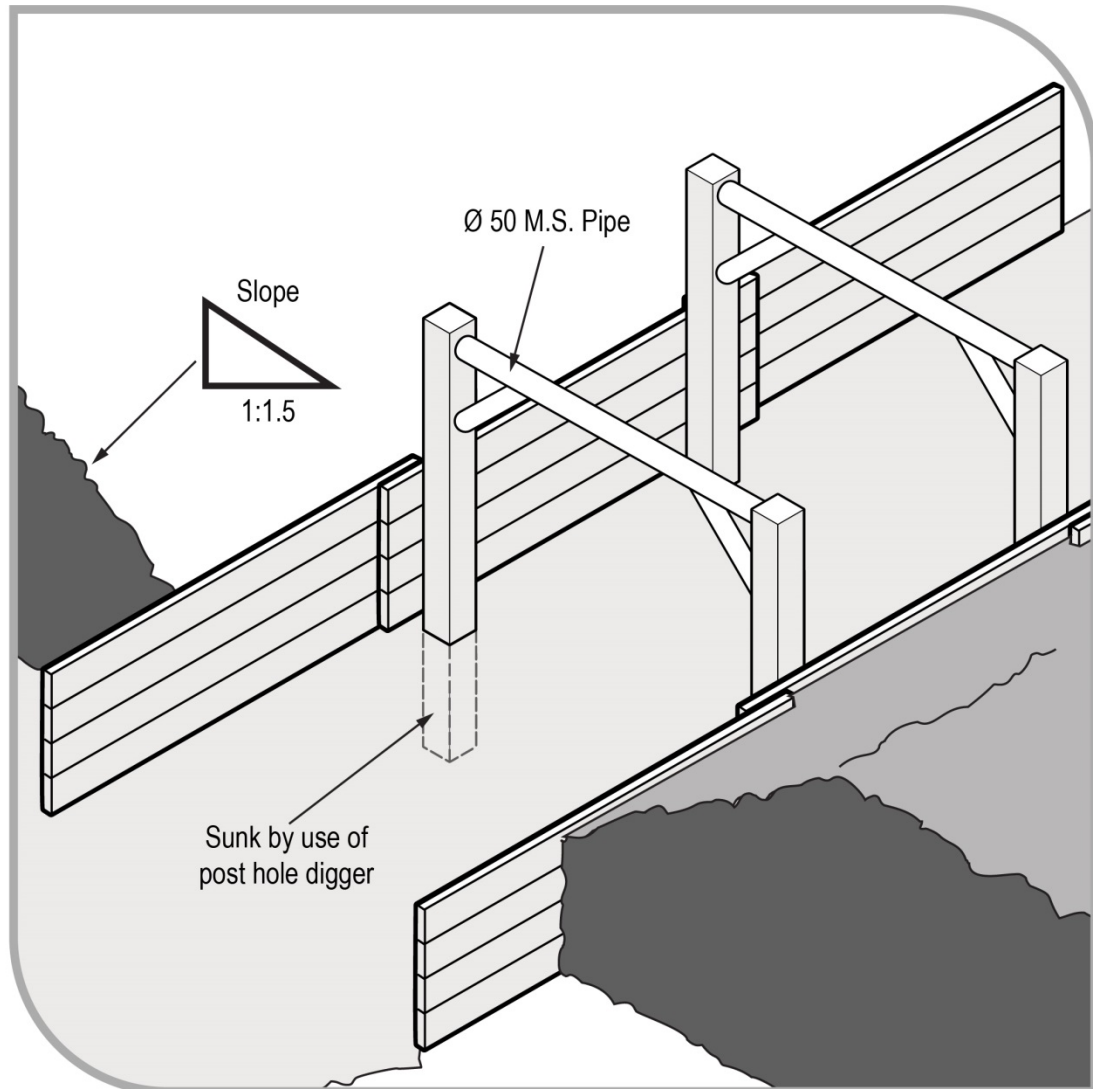
Figure 17 Side lacing in sand trench
