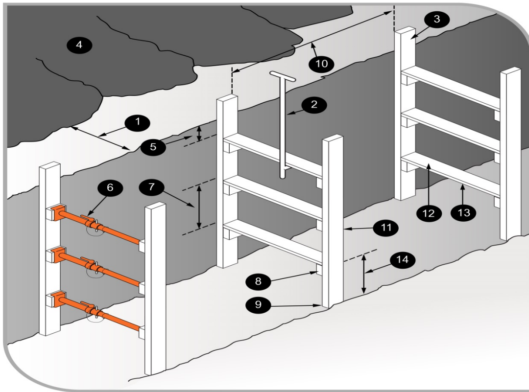
Figure 15 Timber soldier sets
