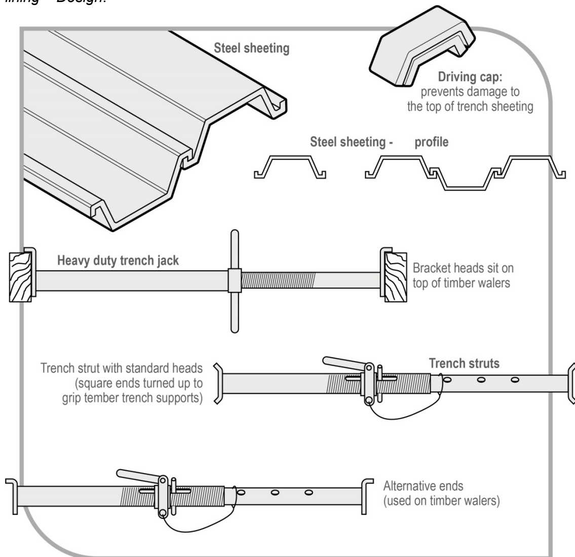
Figure 14 Steel trench sheeting and jacks
