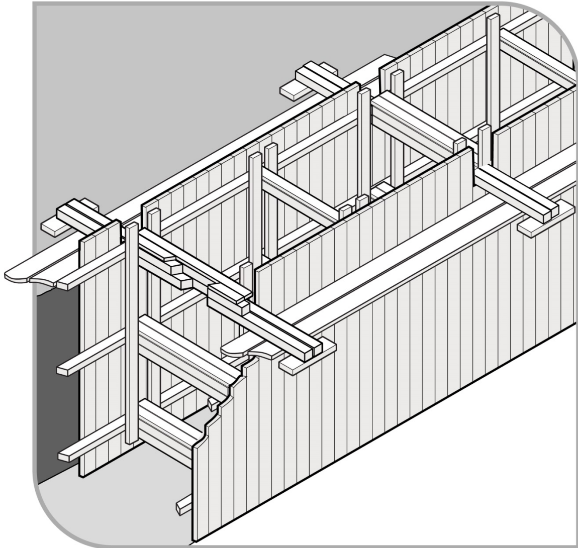
Figure 16 Example of closed sheeting
