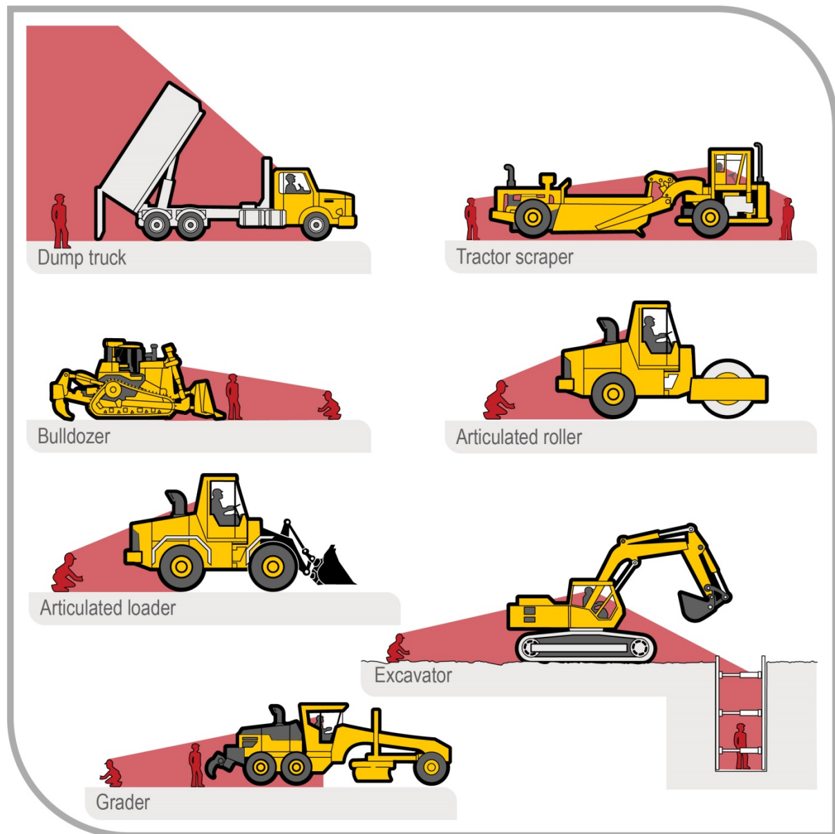
Figure 4 Mobile plant operator blind spots
